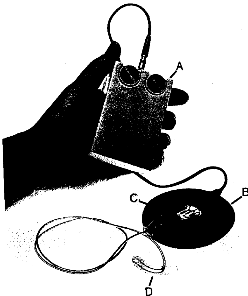
FIG. 1. Peripheral nerve stimulator system consisting of A. external transmitter 455-KHz pulse-modulated carrier sufficient to develop 8-v stimulus at receiver through coupling distance of 1 cm, B. antenna, C. receiver encased in epoxy and coated with thin medical-grade silicone rubber to reduce foreign body reaction and D. wraparound nerve electrode using platinum tinsel wire.
